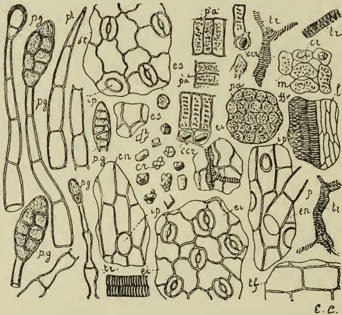
FIG. 80.—Powdered Henbane Leaves. ccr , crystal cells; cr , crystals of calcium oxalate; ei , lower epidermis; es , upper epidermis; fv , portion of fibrovascular bundle of midrib; ip , scar of fallen hair; m , spongy parenchyma; p , portion of hair; pa , p'a' , palisade cells; pg , glandular hairs; pt , simple hairs; st , stomata; tr , cortical parenchyma of midrib; tr , tracheids and vessels. \times 240 . (Greenish and Collin.)
